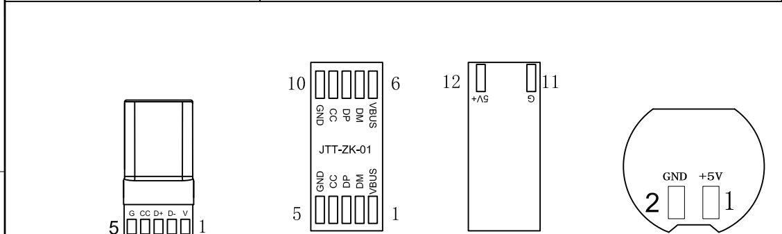
P1/P3 Weld Symbol Drawing P2 Weld Symbol Drawing P4 Weld Symbol Drawing
